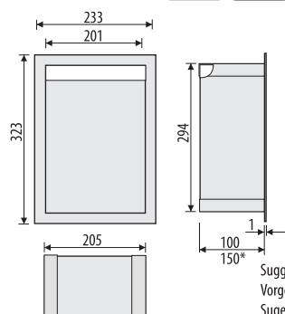
EPWN 200/10 LED EPWN 200/15 LED*
