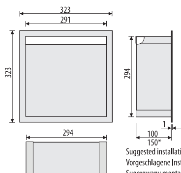
EPWN 300/10 LED EPWN 300/15 LED*
