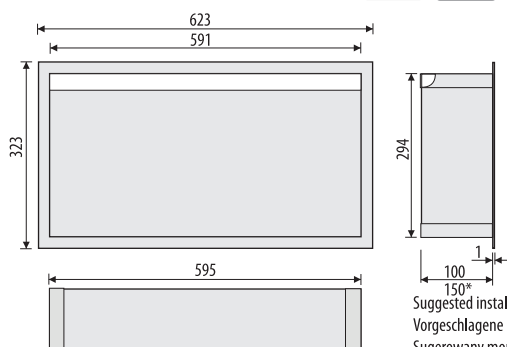
EPWN 600/10 LED EPWN 600/15 LED*
